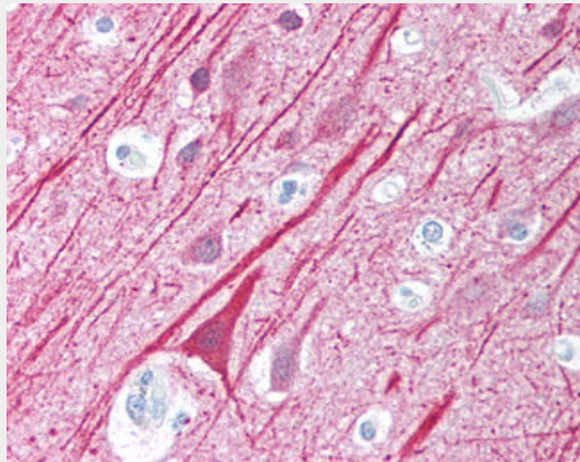
Anti-MAVS antibody IHC of human brain, cortex.
